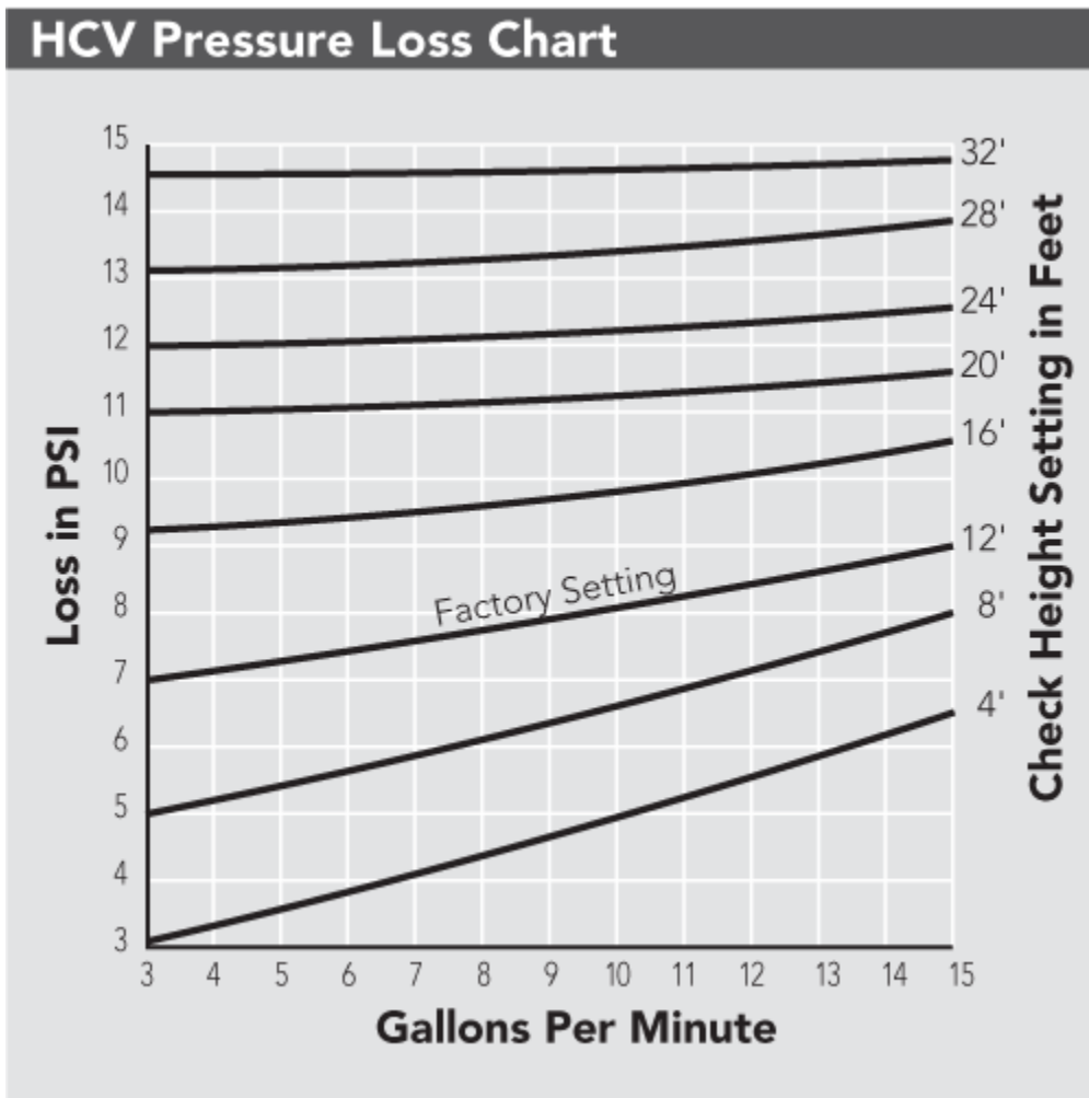
HCV Pressure Loss Chart
