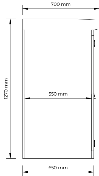
Recommended base installation
