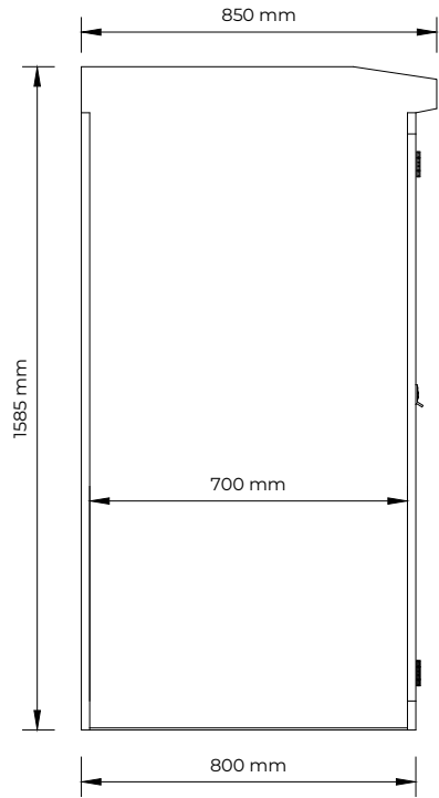
Recommended base installation
