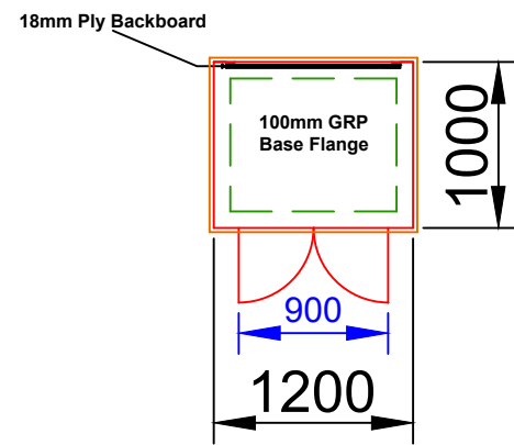
ENCLOSURE PLAN VIEW 1
