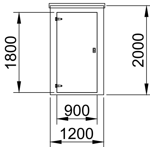
EXTERNAL ELEVATION WALL 1 (FRONT WALL)
