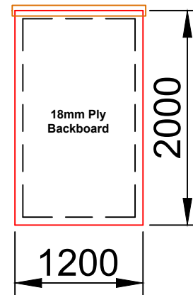
ENCLOSURE REAR VIEW 4
