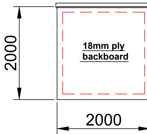
External Elevation WALL 3
