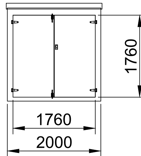
External Elevation WALL 1
