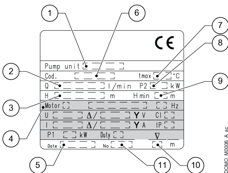
Figure 2: Three-phase
