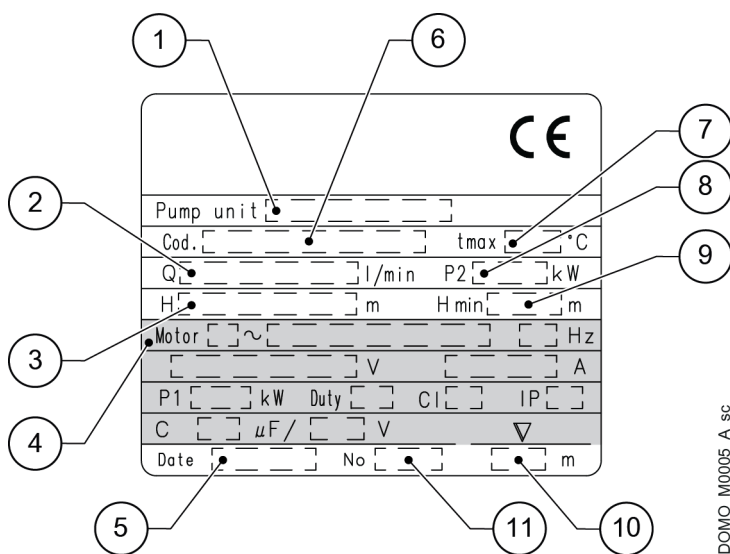
Figure 1: Single-phase
