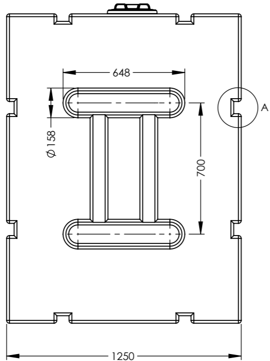
LEFT VIEW
