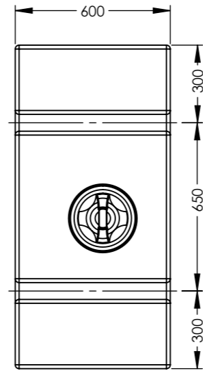
PLAN VIEW
