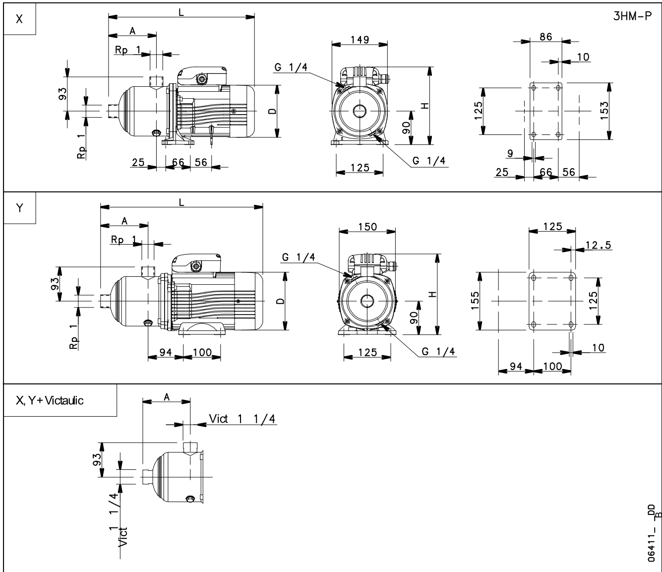
Dimensions mm
